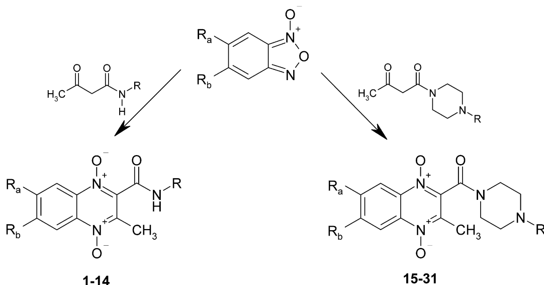
Scheme 1. Synthesis of compounds 1–31 .
