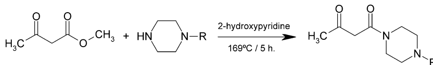
Scheme 2. Synthesis of the intermediates N -(3-oxobutyl)-piperazine derivatives.
